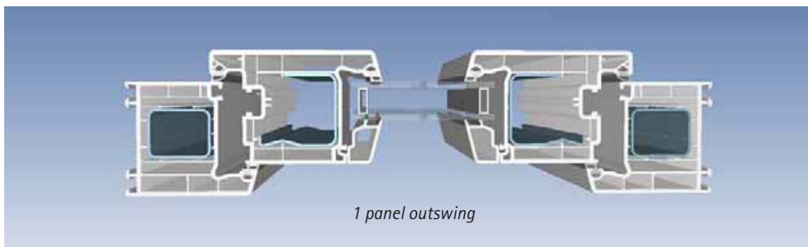
1 panel inswing
